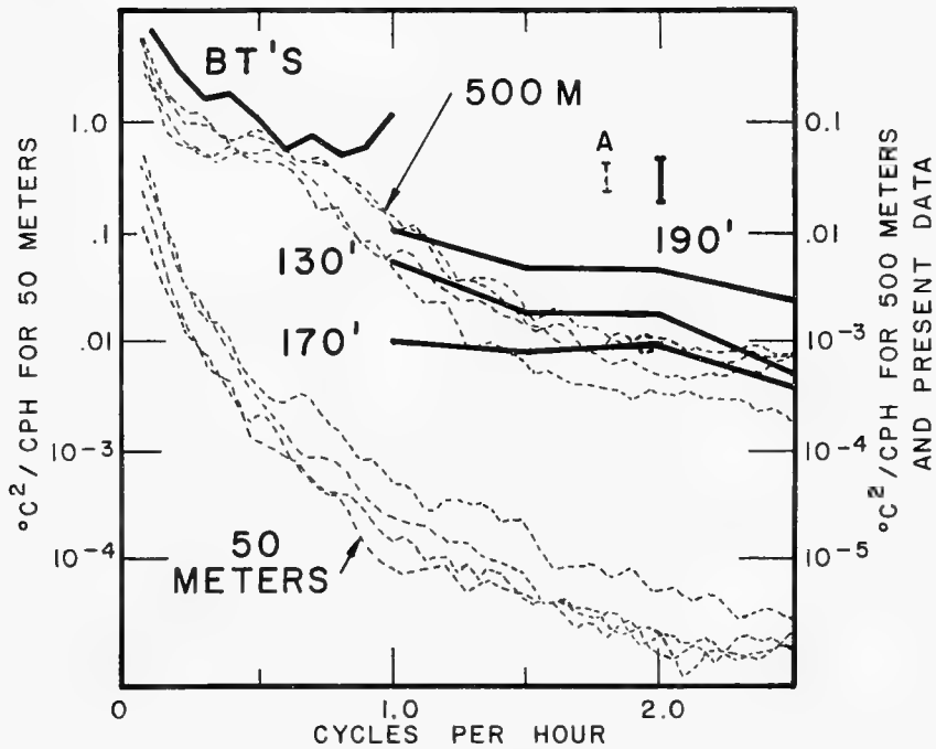
Figure 9. Comparison of power spectra of temperature fluctuations obtained by thermistors at Bermuda 2 (dotted lines) and by thermometer units at Eleuthera (solid lines). The corresponding estimates of error are given by the error bars.
